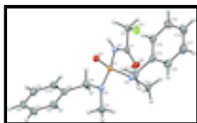
Fig. 1. The molecular structure of the title compound with ellipsoids shown at the 50% probability level.
